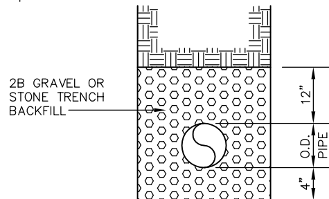
TRENCH SECTION
